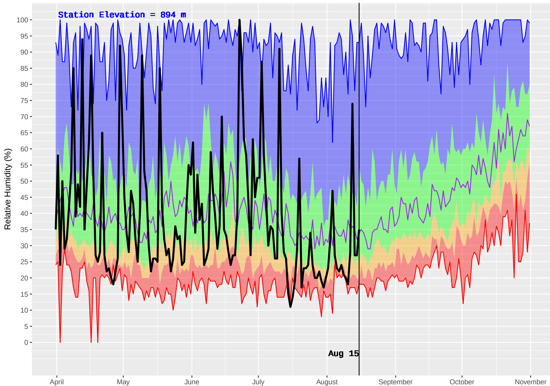
TOBY HUB (417) : Historical (1986–2016) and Current (2018) Daily Relative Humidity
