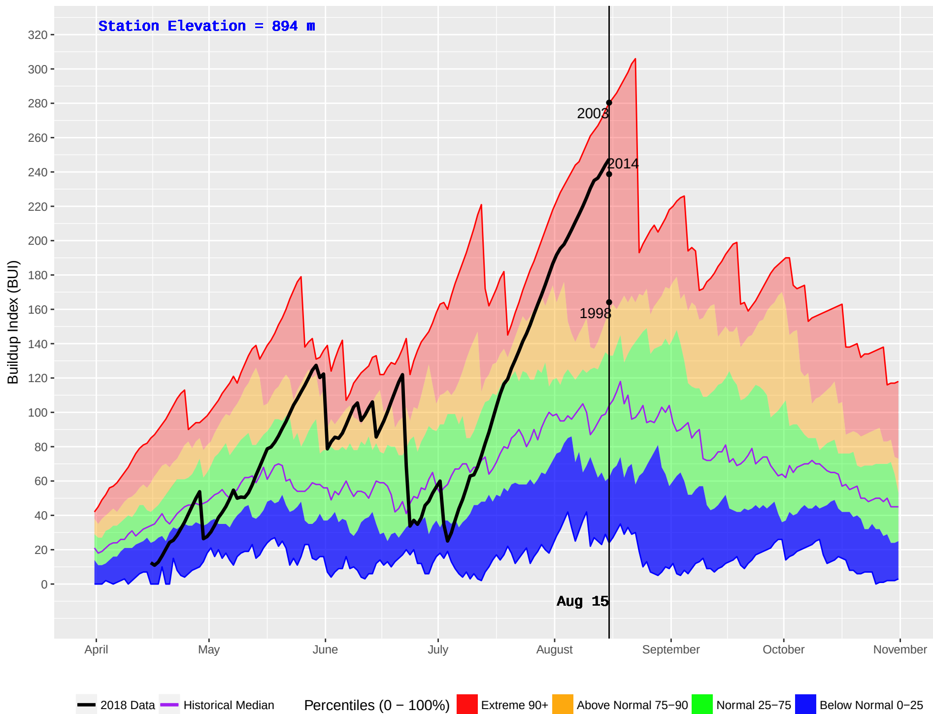
TOBY HUB (417) : Historical (1986–2016) and Current (2018) Daily Buildup Index (BUI)
