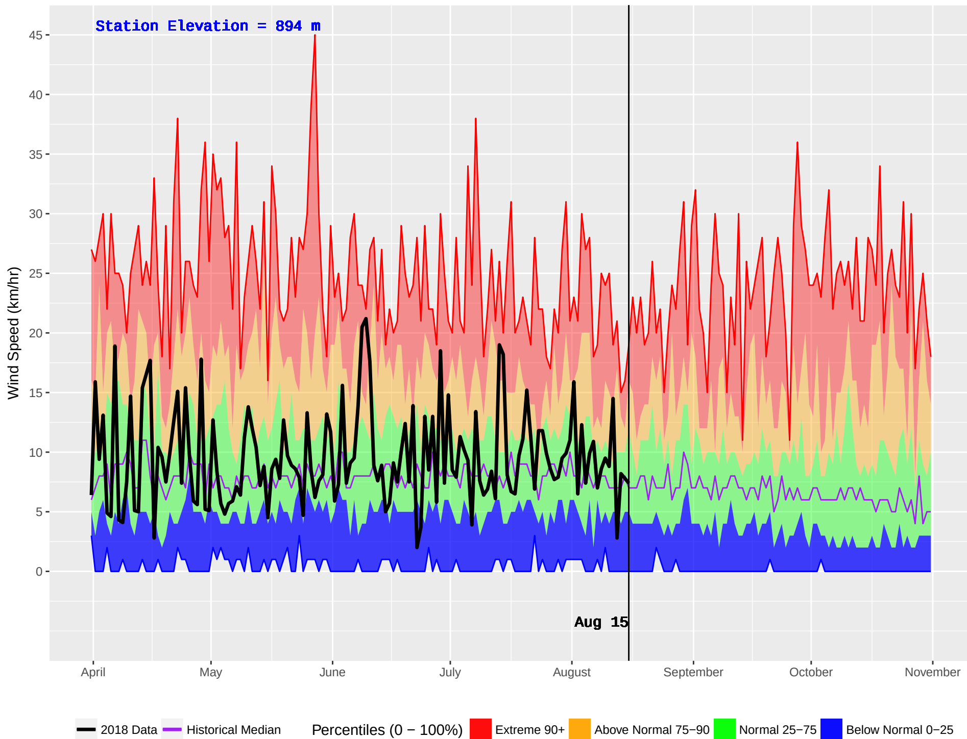
TOBY HUB (417) : Historical (1986–2016) and Current (2018) Daily Wind Speed
