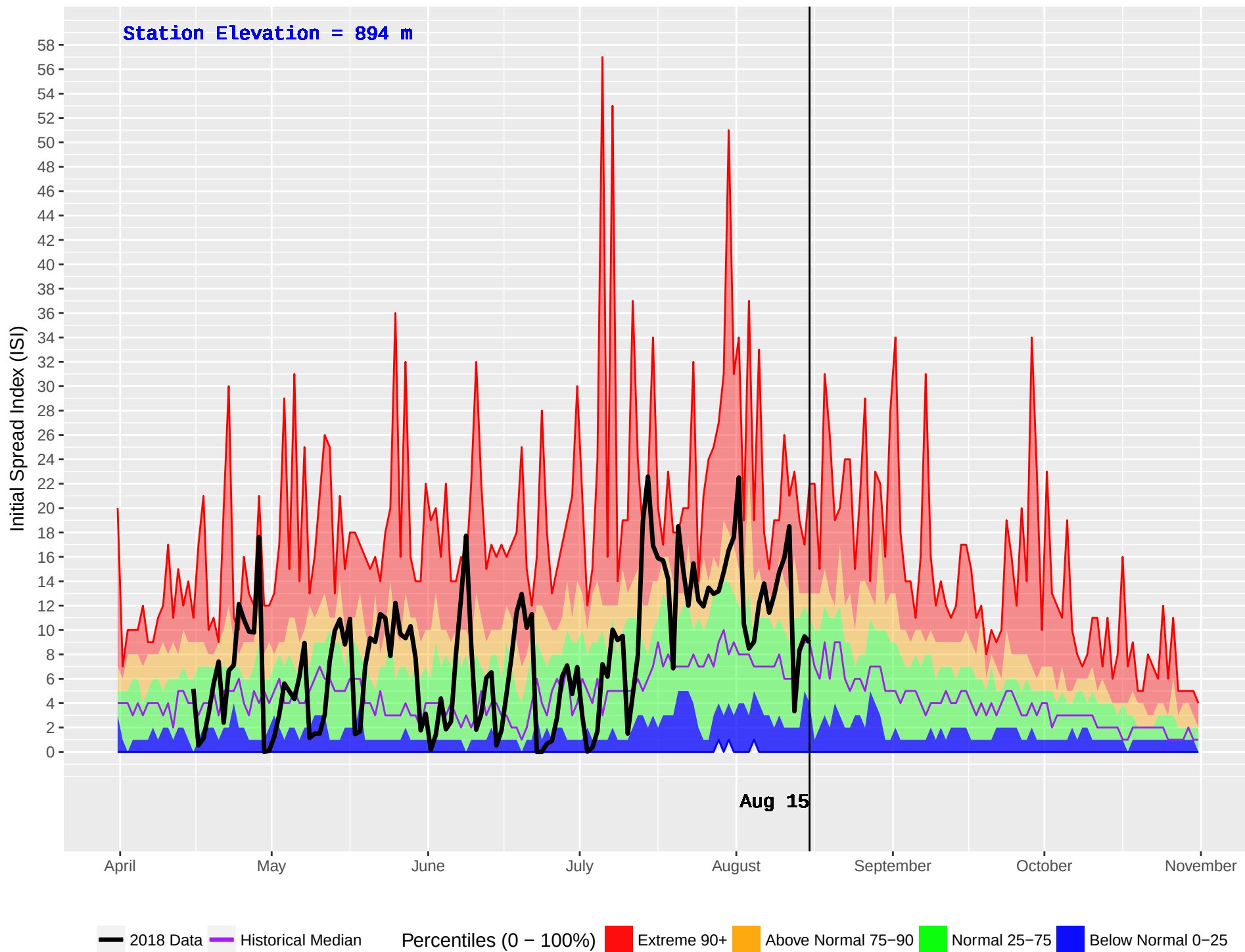
TOBY HUB (417) : Historical (1986–2016) and Current (2018) Daily Initial Spread Index (ISI)
