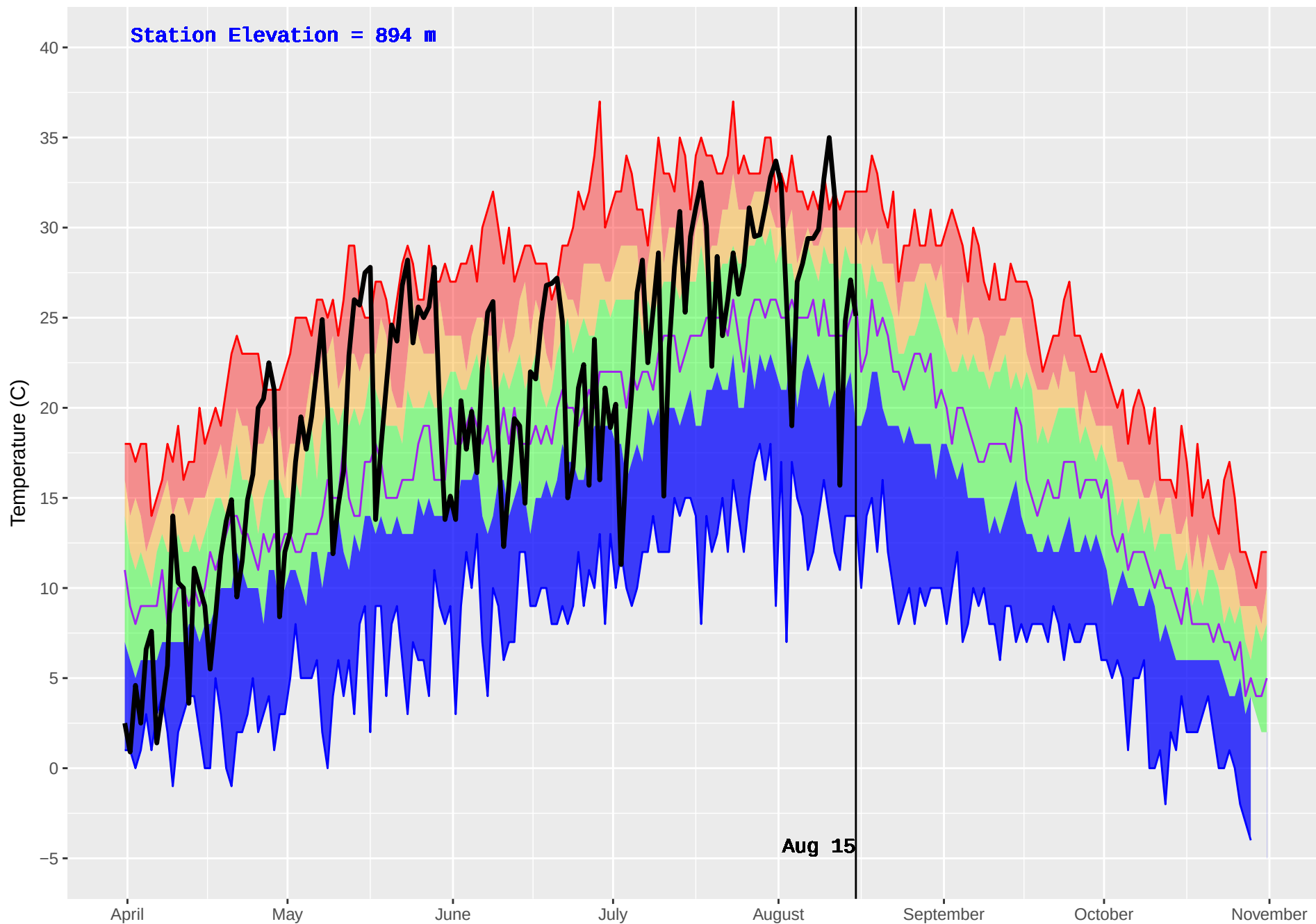
TOBY HUB (417) : Historical (1986–2016) and Current (2018) Daily Temperature
